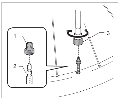
► 1. Presta valve adapter 2. Valve stem 3. Air chuck
